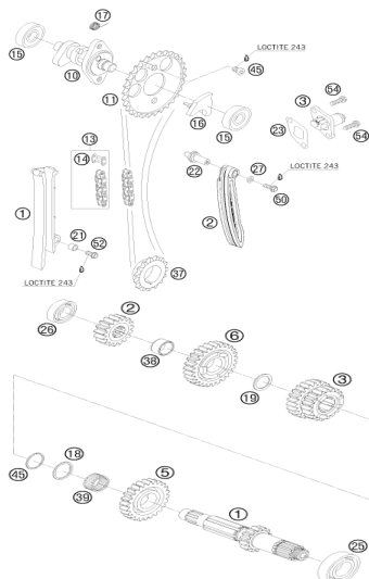
Timing drive
