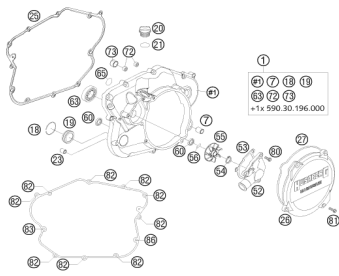
Clutch cover
