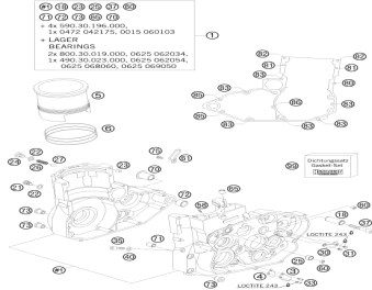
Engine case
