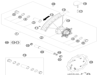
Front wheel
