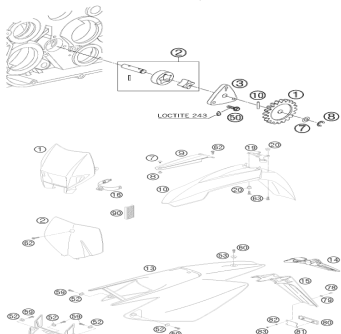
Lubricating system
