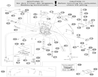
Carburetor
