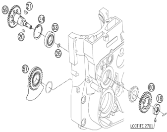
Balancer shaft
