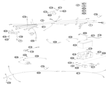
Wiring harness
