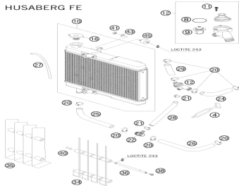
Cooling system
