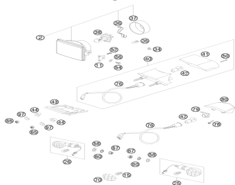
Lighting system
