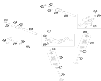
Valve drive
