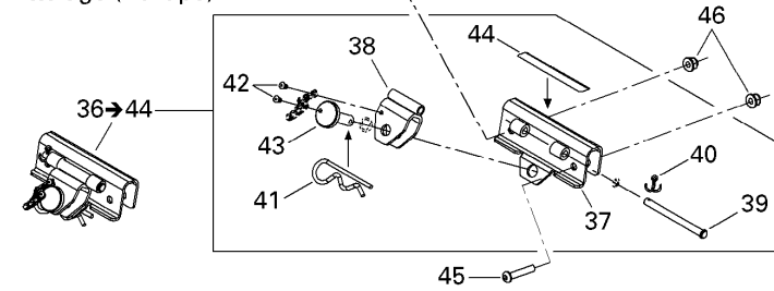
Hitch (Europe)/ Attelage (Europe)
